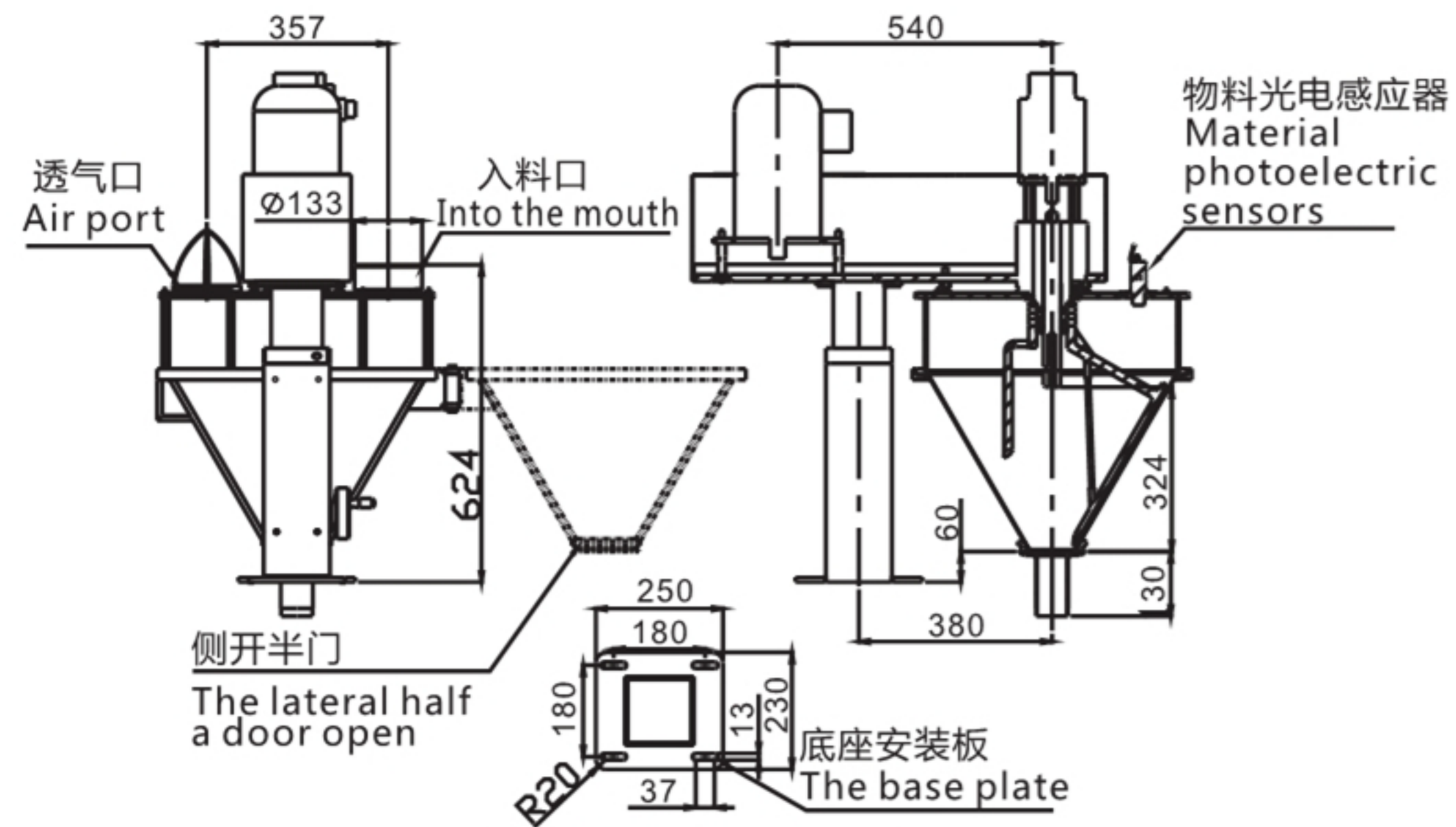
JA-50L螺杆计量机 (平顶ceiling Screw measuring machine)
